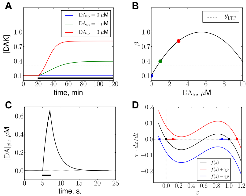
Fig. 2. Overview of the main components of the model. (A) Evolution of [DAK] at bath DA concentrations [DA]_{to} = 0 \mu\text{M} (blue line), [DA]_{to} = 1 \mu\text{M} (green line) and [DA]_{to} = 3 \mu\text{M} (red line). The thick black line denotes the period of the DA bath. The dashed line denotes the threshold for LTP ( \theta_{LTP} ). (B) Function \beta([DA]_{to}) describes the modulation of the rate of [DAK] activation by tonic DA (see Eq. (2)). Colored dots mark the value of \beta for tonic DA concentrations equal to 0, 1, and 3 \mu\text{M} . (C) Phasic DA release in \mu\text{M} induced by 2 s 50 Hz stimulation. Black bar denotes stimulation time. (D) Dynamics of the z variables. In the absence of stimulation the fixed points of the synaptic state are z = 0 (depression) and z = 1 (potentiation), marked by the black dots. If the synapse is tagged for LTP ( h_n = 1 ) and p > 0 , z can pass from depression for potentiation (corresponding to the movement of the phase point from the left black dot towards the red dot). For the LTD tag ( h_n = 1 ), a synapse potentiated earlier can pass to the depressed state (corresponding to the movement of the phase point from the right black dot towards the blue dot).
